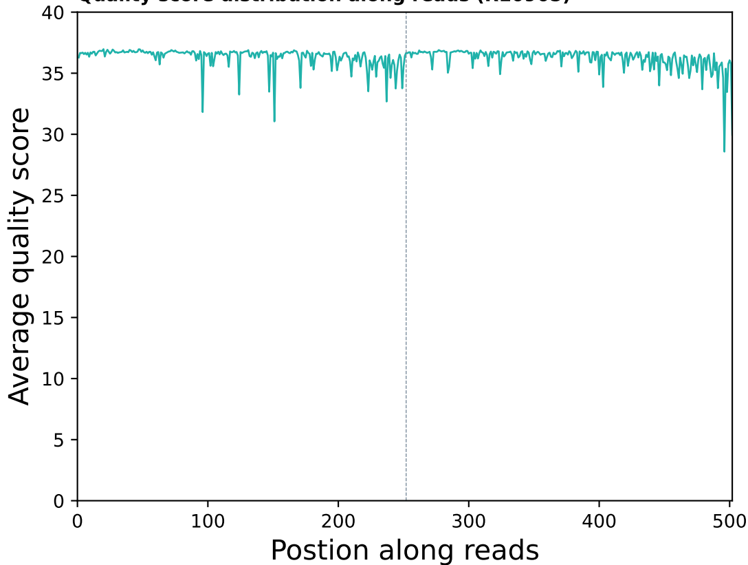
Quality score distribution along reads (R10905)
